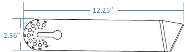
Flood Mount Bracket (ENC FLMT)
