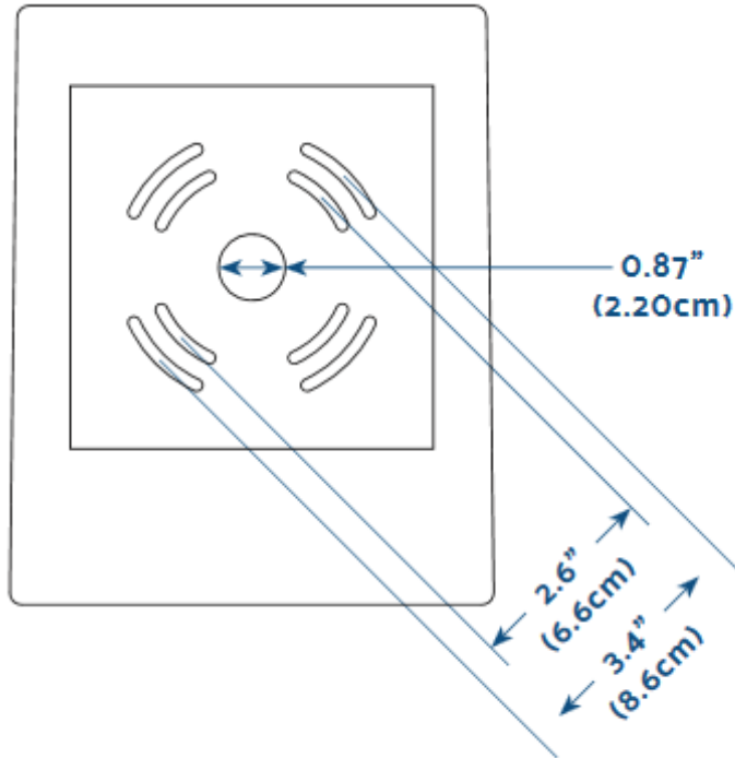
30W Fixture
